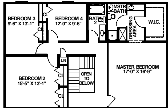
SECOND FLOOR PLAN 1344 S.F.
