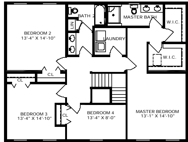
SECOND FLOOR PLAN 1260 S.F.
