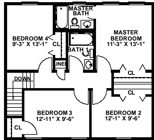
SECOND FLOOR PLAN 840 S.F.
