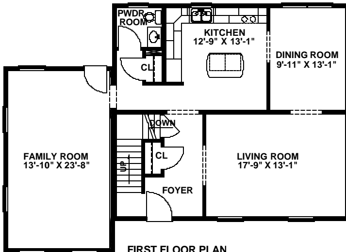
FIRST FLOOR PLAN 1176 S.F. (with morning room)
