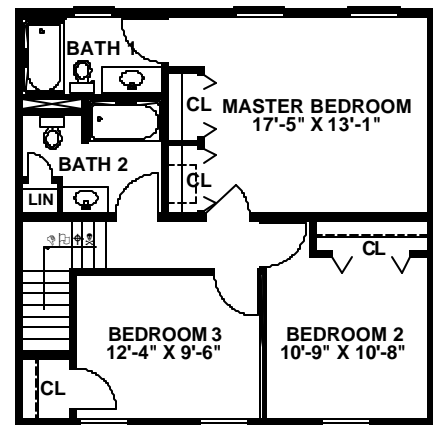
SECOND FLOOR PLAN 784 S.F.
