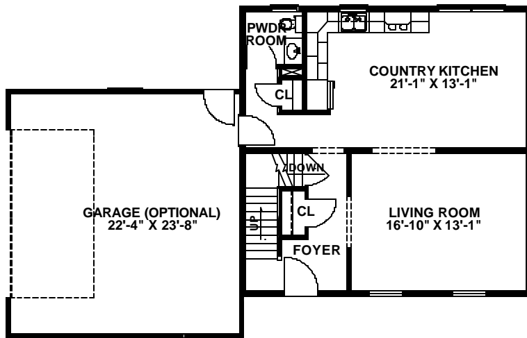
FIRST FLOOR PLAN 784 S.F.
