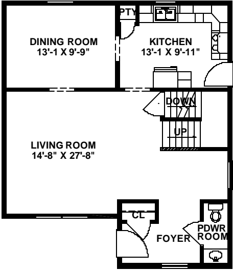
FIRST FLOOR PLAN 812 S.F.
