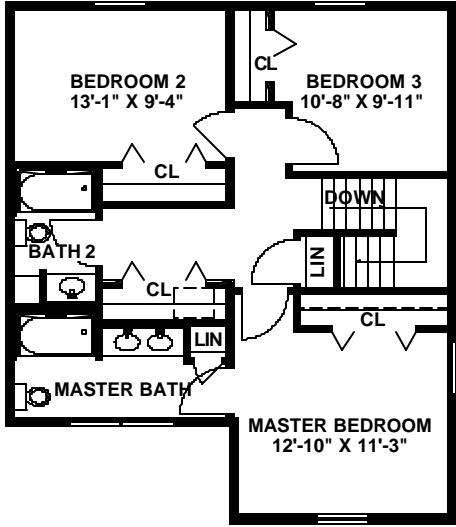
SECOND FLOOR PLAN 812 S.F.
