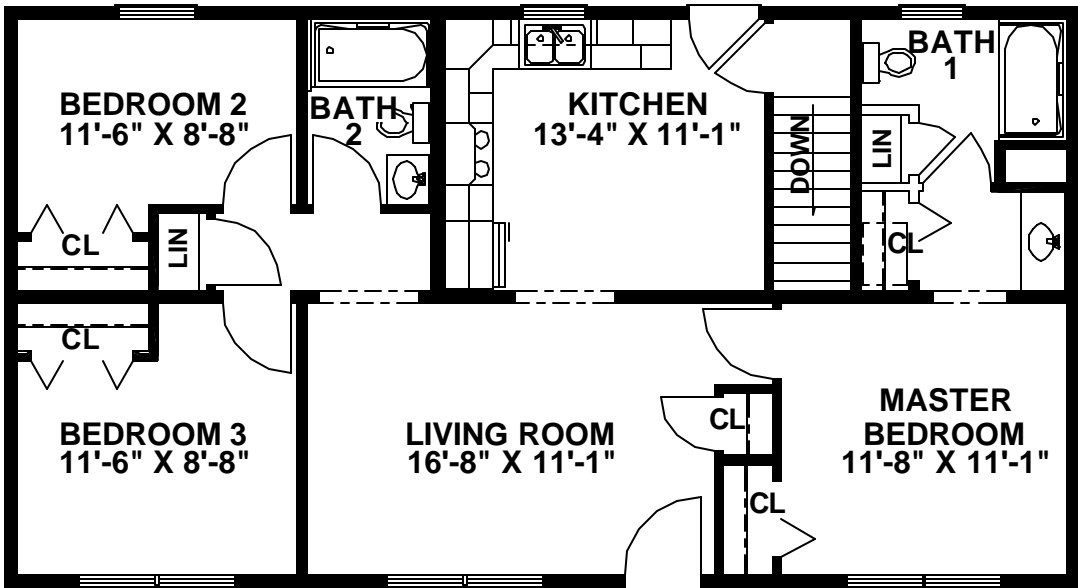
FLOOR PLAN 1056 S.F.
