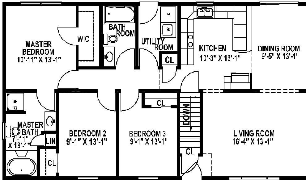
FLOOR PLAN 1344 S.F.
