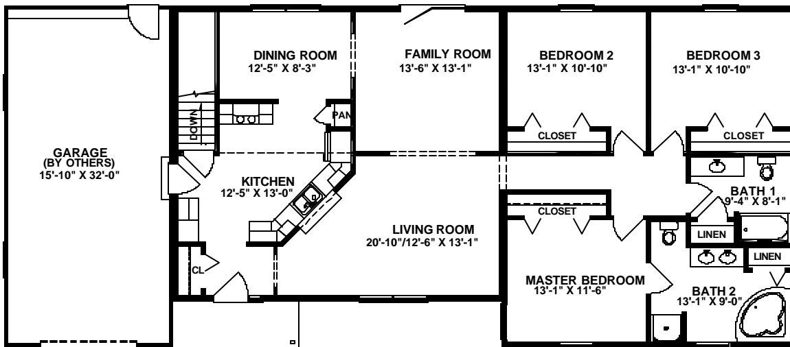
FLOOR PLAN 1762 S.F.
