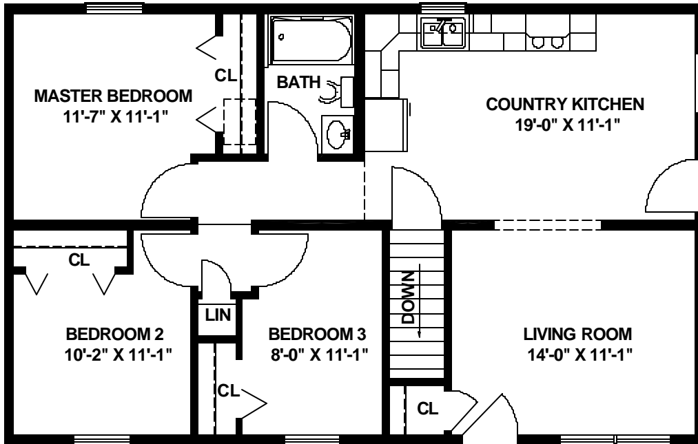
FLOOR PLAN 960 S.F.
