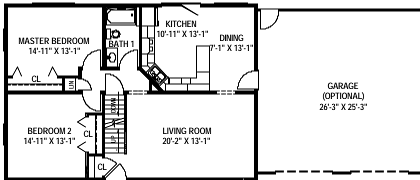
FIRST FLOOR PLAN 1064 S.F.
