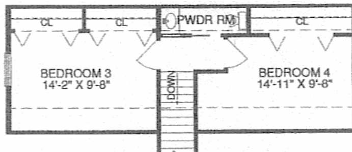
OPTIONAL SECOND FLOOR PLAN
