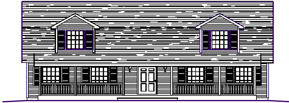
FRONT ELEVATION OVERALL DIMENSIONS: 40'-0" x 28'-0"
