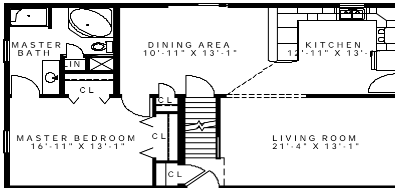
FIRST FLOOR PLAN 1120 S.F.
