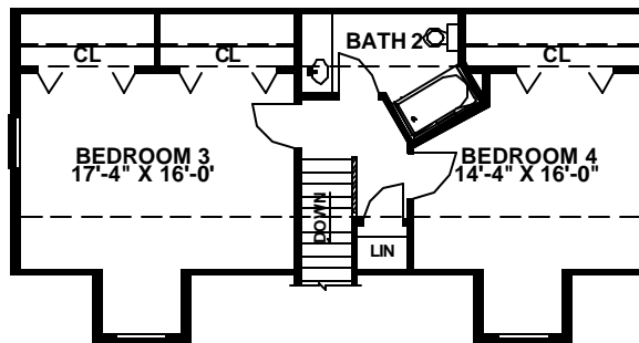
OPTIONAL SECOND FLOOR PLAN
