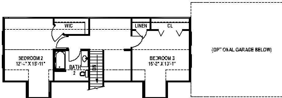
OPTIONAL SECOND FLOOR PLAN 775 S.F.
